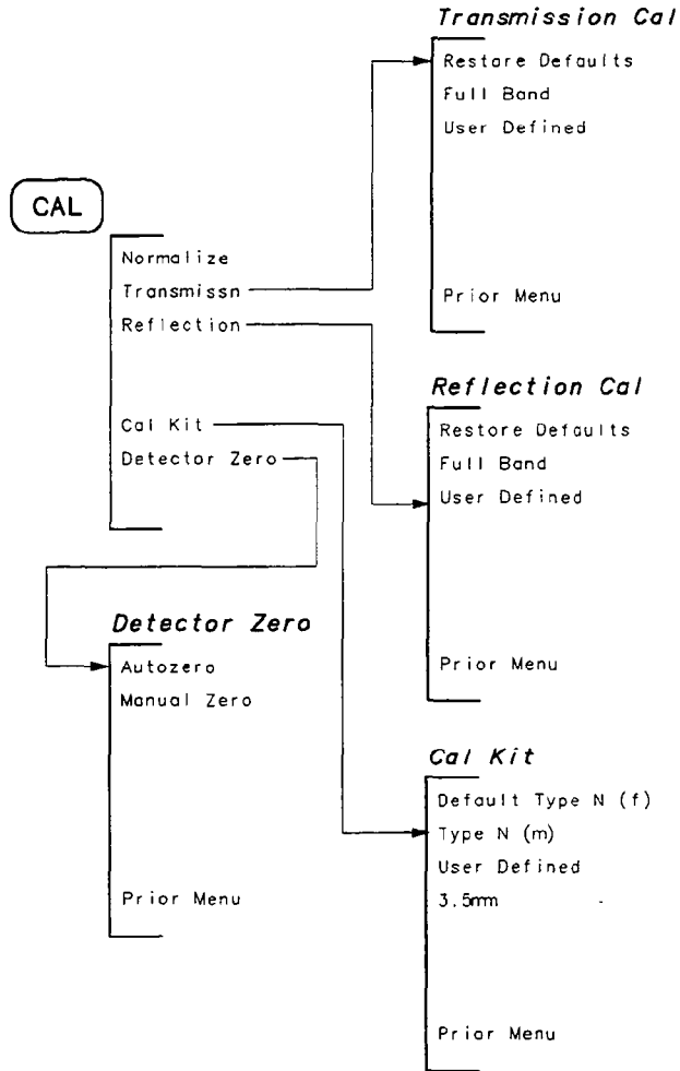
Figure 7-3. Calibration Menu
