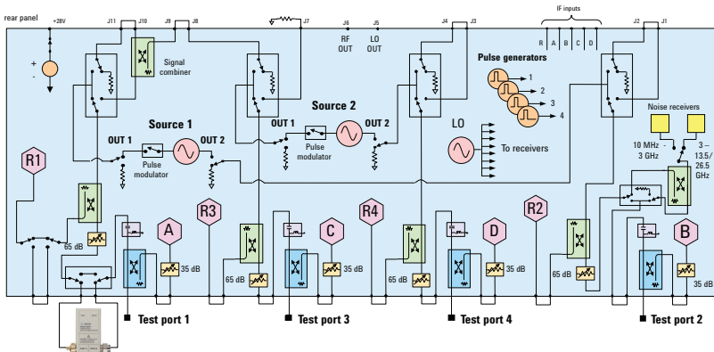
N5241/42A 4-port block diagram with noise figure option
